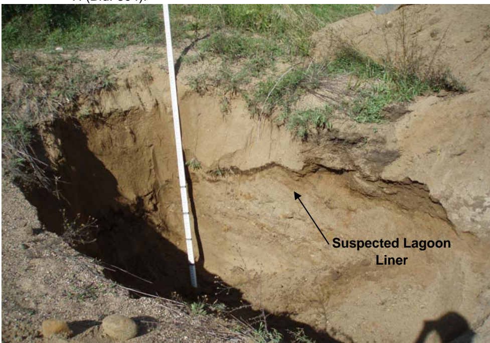
Photo 10 Test trench SOC5-TT29 in the former rinsate lagoon. Lagoon liner was observed in this test trench.
