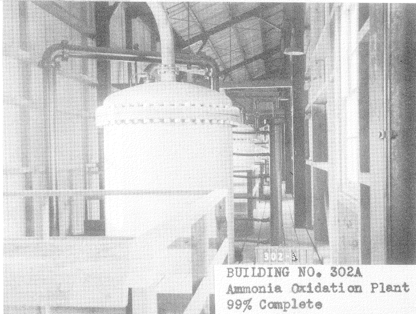
BUILDING NO. 302A Ammonia Oxidation Plant 99% Complete
