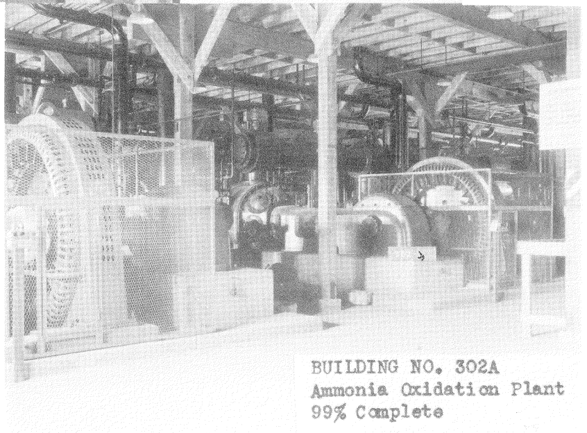
BUILDING NO. 302A Ammonia Oxidation Plant 99% Complete
