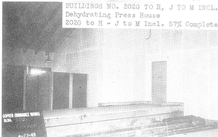
BUILDINGS NO. 202G to H, J TO M INCL. Dehydrating Press House 202G to H - J to M Incl. 57% Complete
