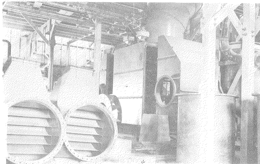
BUILDING NO. 251A Act. Carb. Solv. Recov. System 48% Complete
