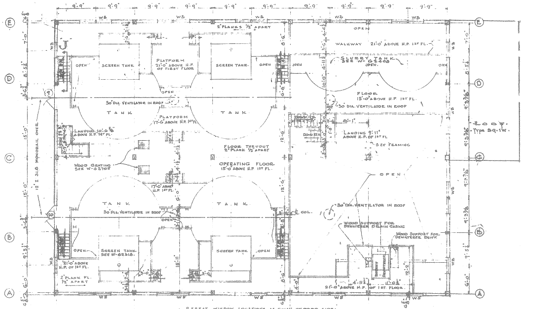
OPERATING FLOOR PLAN
