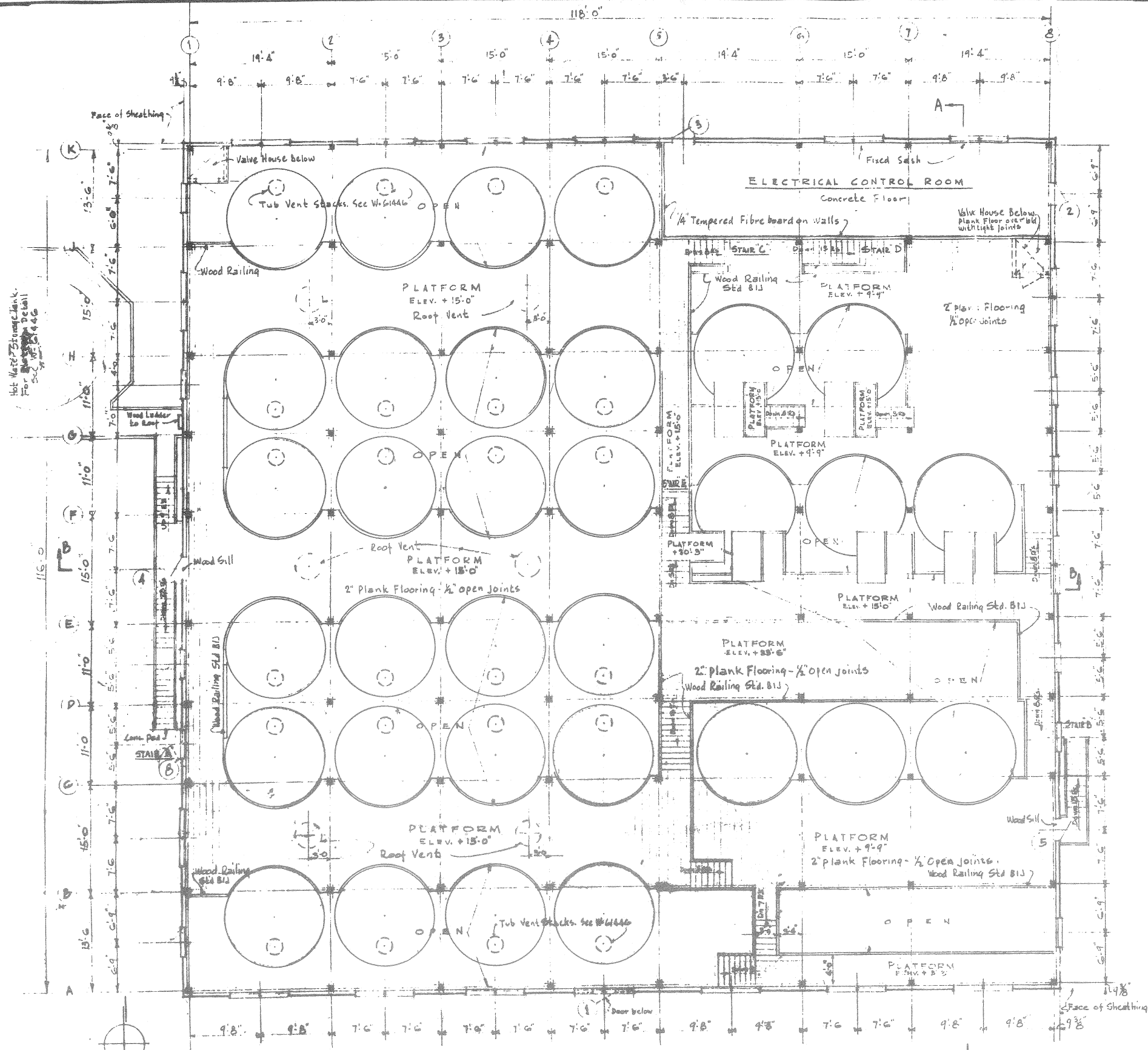
OPERATING FLOOR PLAN
