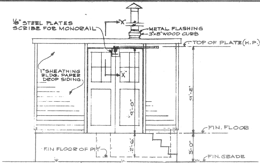
PLATFORM ELEVATION SCALE \frac{1}{4} "=1'-0"
