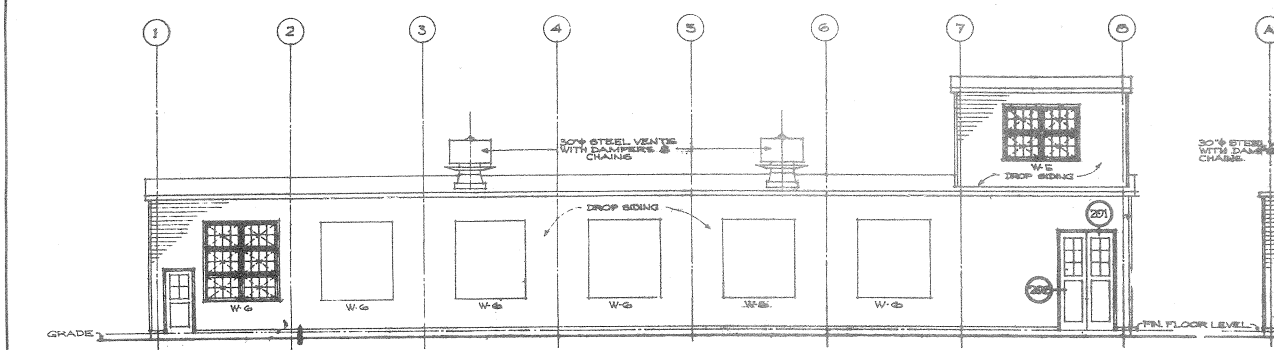
ELEVATION 1-1 1/8" = 1'-0"
